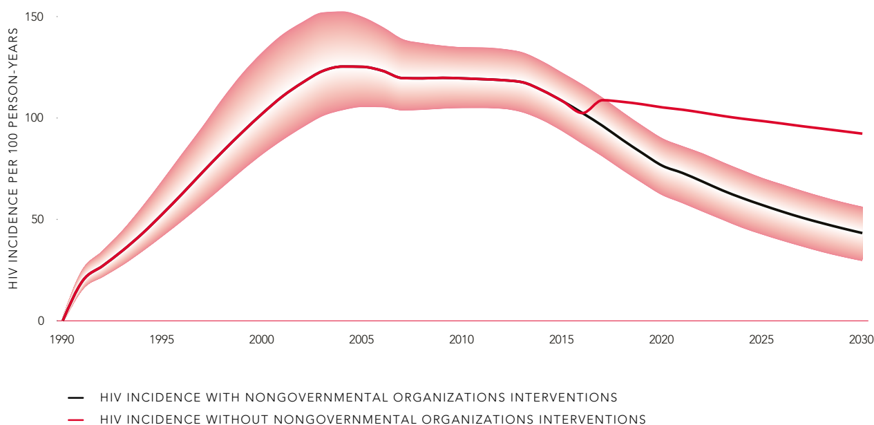
FIGURE 2.10 HIV incidence among gay men and other men who have sex with men, modelled with and without nongovernmental organization interventions, Ukraine, 1990–2030
