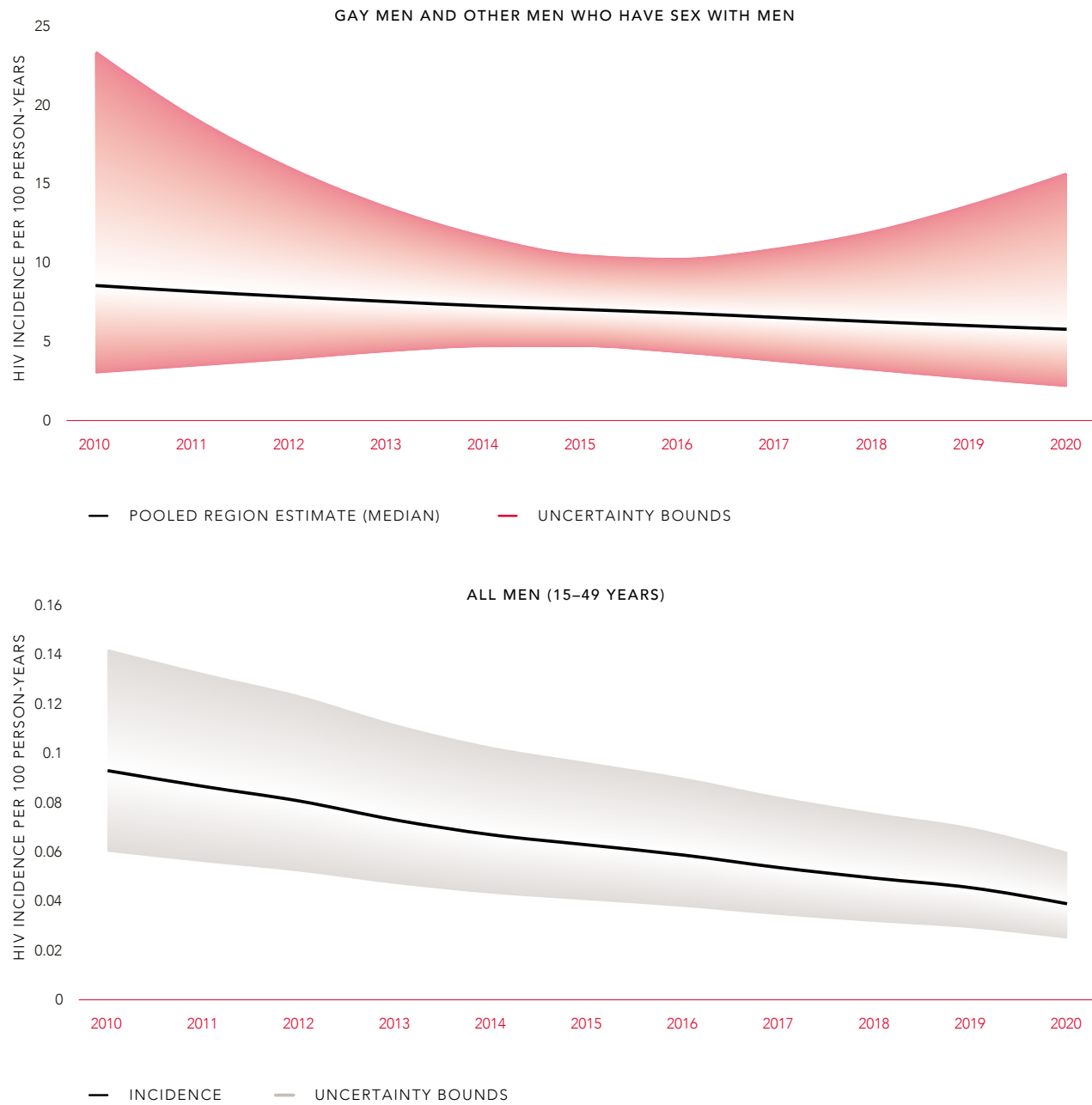
FIGURE 2.2 Estimated HIV incidence among gay men and other men who have sex with men and all adult men (15–49 years) in the general population, western and central Africa, 2010–2020
